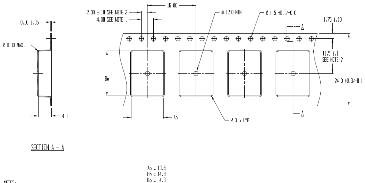
Figure 14: NINA-B111 tape dimensions
